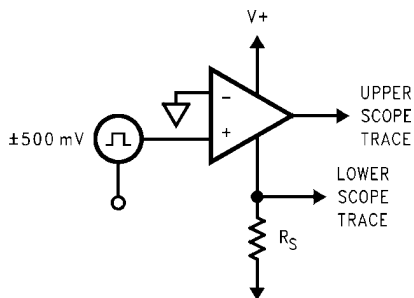
FIGURE 5. R_S = 10\Omega
