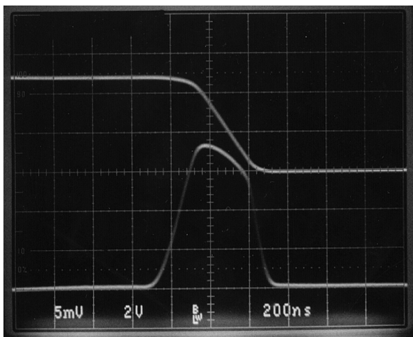
FIGURE 5. R_S = 10\Omega
